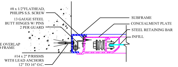
C TYP. SCREEN DETAIL @ HINGE
