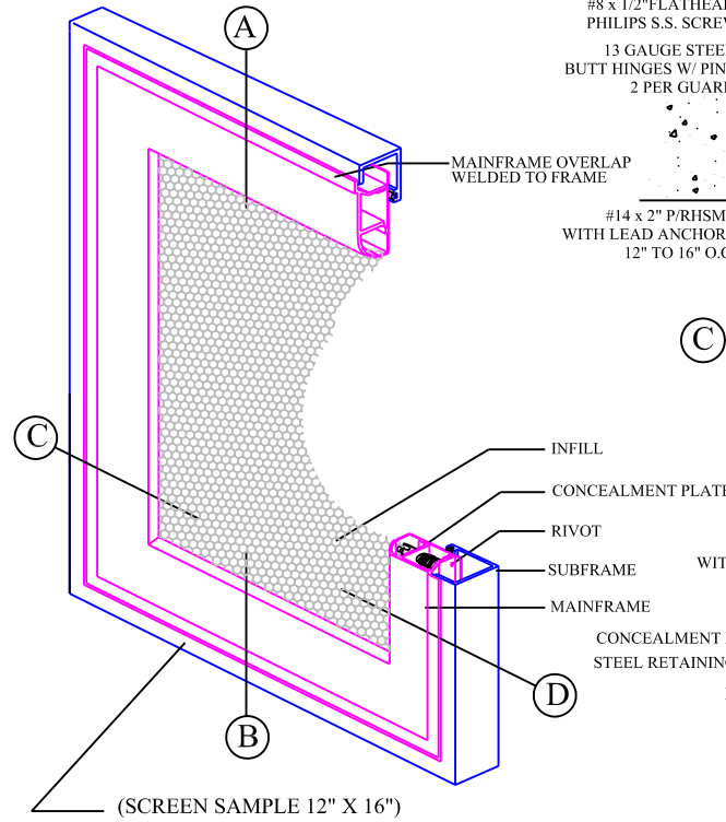
A TYP. SCREEN DETAIL @ HEAD
