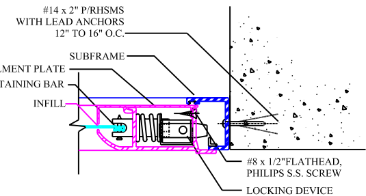
D TYP. SCREEN DETAIL @ LOCK
