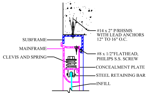
A TYP. SCREEN DETAIL @ HEAD
