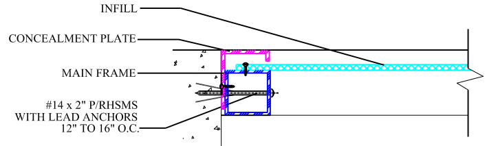
D JAMB DETAIL @ BOTH SIDES
