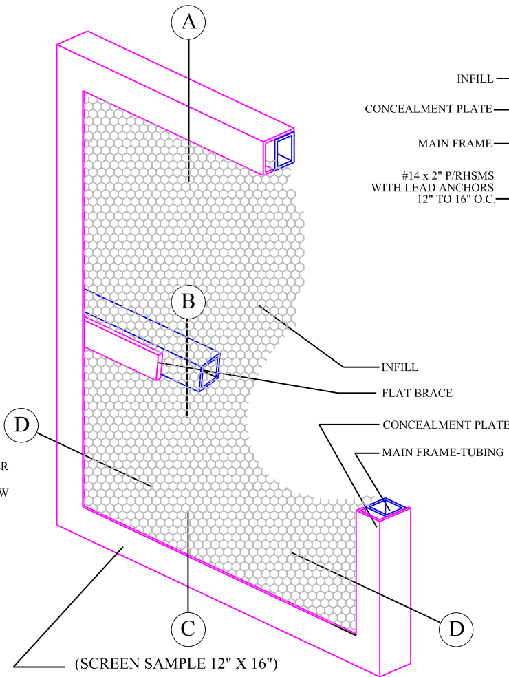
D JAMB DETAIL @ BOTH SIDES
