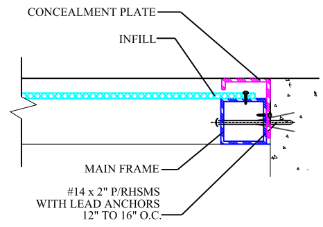
D JAMB DETAIL @ BOTH SIDES
