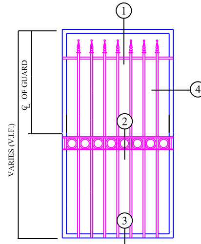
STEEL ARCHITECTURAL BAR GUARD ELEVATION
