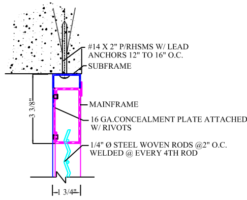
A TYP. JAMB DETAIL @ HEAD
