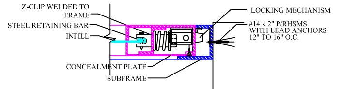
C TYP. SCREEN DETAIL@ HINGE
