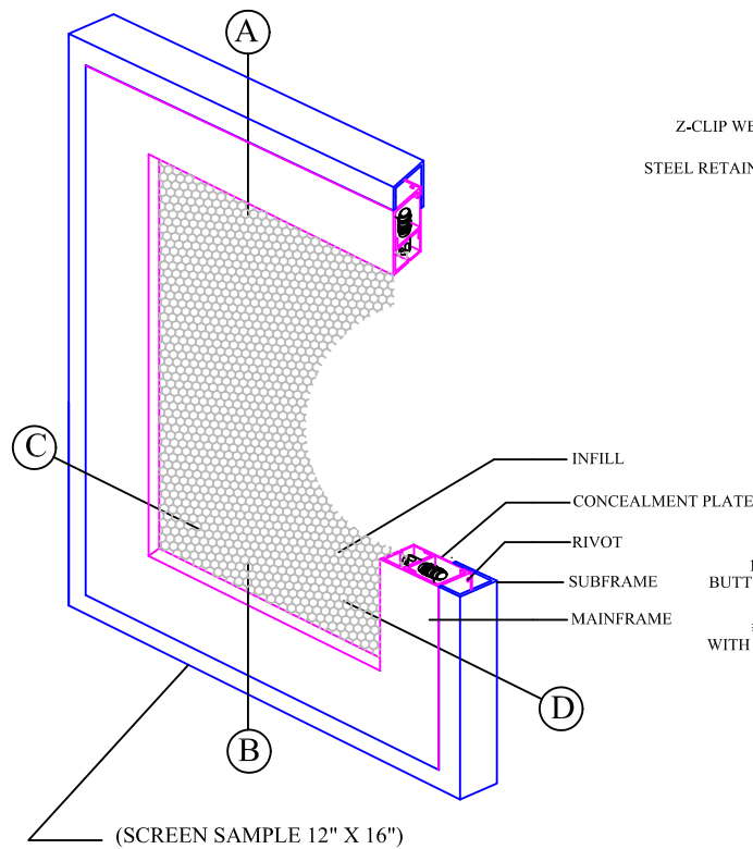
C TYP. SCREEN DETAIL@ HINGE
