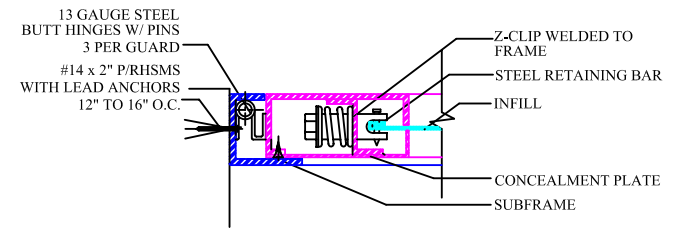
D TYP. SCREEN DETAIL@ LOCK
