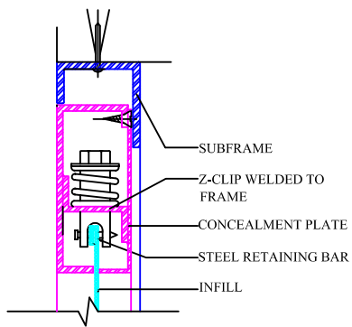
A TYP. SCREEN DETAIL@ HEAD
