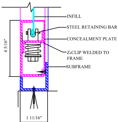
B TYP. SCREEN DETAIL@ SILL
