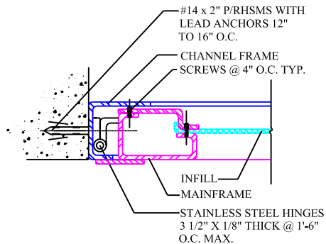
E TYP. SCREEN DETAIL@ HINGE
