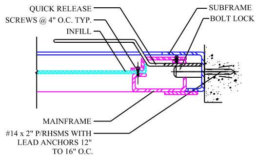
D TYP. SCREEN DETAIL@ LOCK
