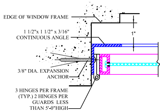
(E) TYP. JAMB DETAIL @ HINGE
